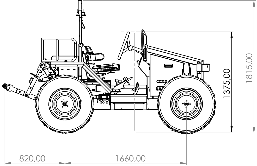
BUGRAY TRACTOR WEIGHT: 650 KG
